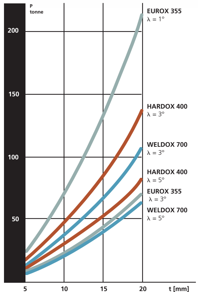
Fig. 3. Shearing force as a function of the thickness and rake angle \lambda
